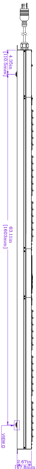
VIEW C
